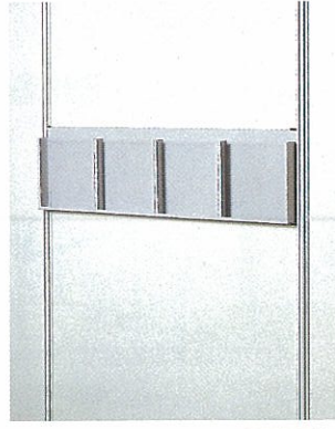
Catalogue Holder CH-02 (metal) 970L X 50D X 280H mm
